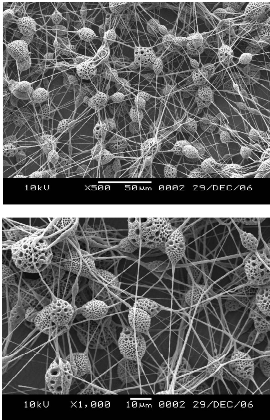
Figure 6: SEM pictures of the electrospun nanoporous microspheres. The flow is 1.5ml/h.
