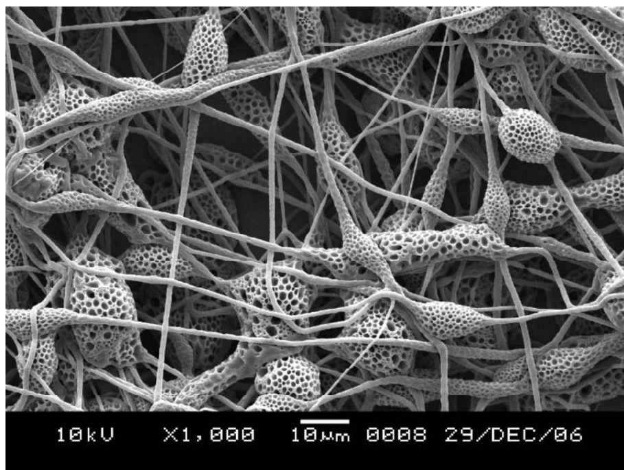
Figure 5: SEM pictures of the electrospun nanoporous microspheres. The voltage is 15KV.
