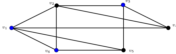
FIGURE 1. Graph G
