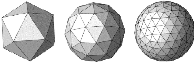
Figure 1: The basic icosahedron and its first two tessellations
