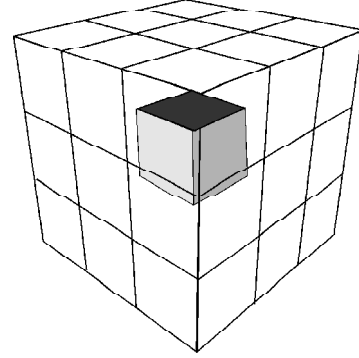
Figure 2: Cubic centered neighborhood
