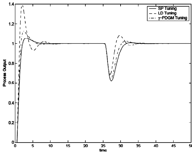
Figure 11: Performance of the Set-point (Solid), Load-disturbance (Dashed) and \gamma -PDGM (Dot-dashed) Tunings, Operating in Both Servo and Regulation Modes
